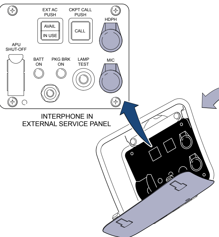
EXTERNAL SERVICE PANEL
